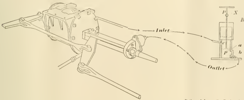
PROPOSED MODIFICATION OF THE SLACK ADJUSTER.
